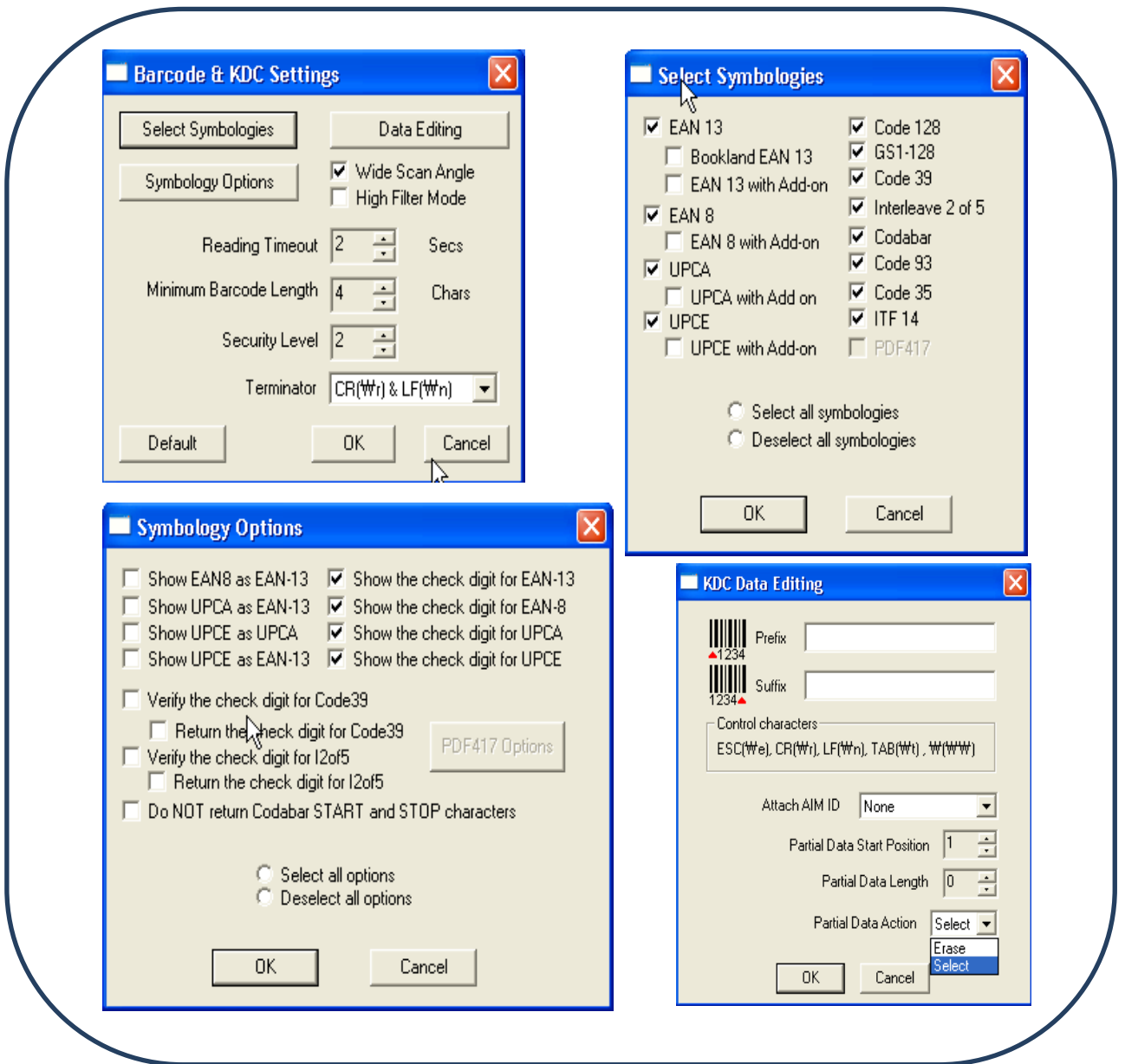
図 28-Barcode & KDC Settings, Symbologies, Data Editing and Scan Options
