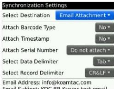
図 34-Blackberry bKTSync
