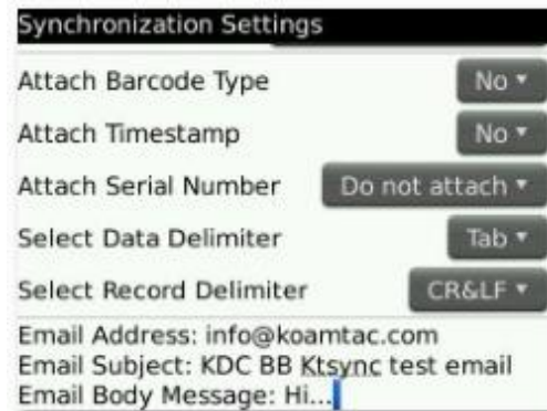
図 34-Blackberry bKTSync
