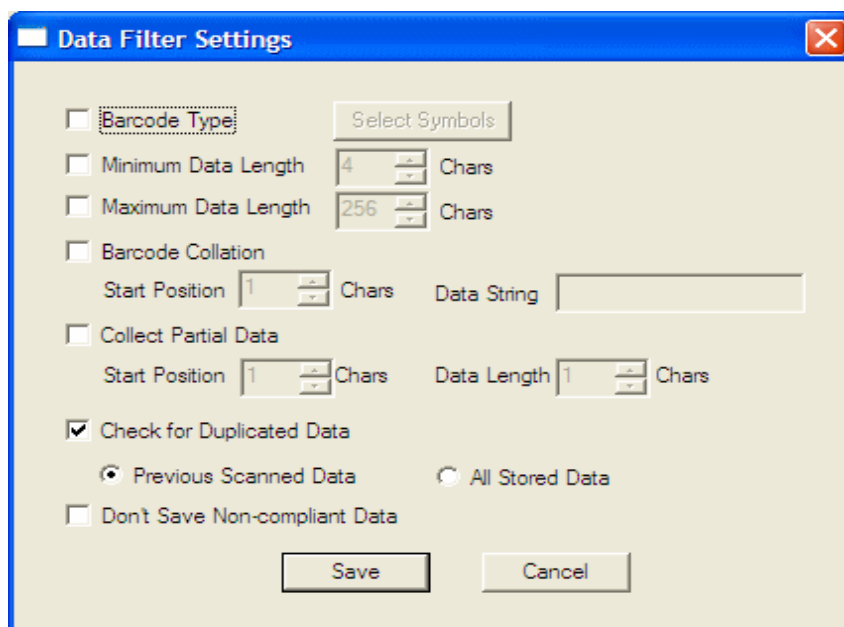
図 38-Data Filter Settings
