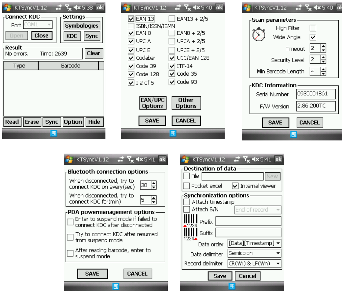
Figure 36 - Mobile pKTSync
