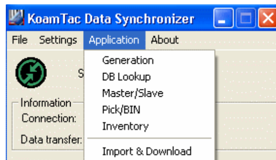
Figure 40 - Application Menu
