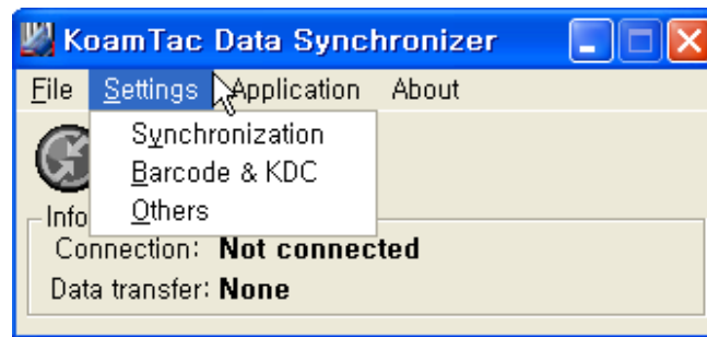
Figure 25 – Setting Menu
