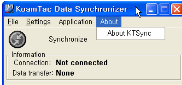
Figure 27 - About Menu
