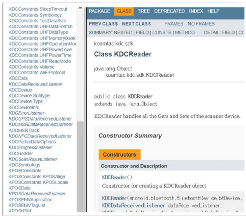
Figure 22 – SDK Package
